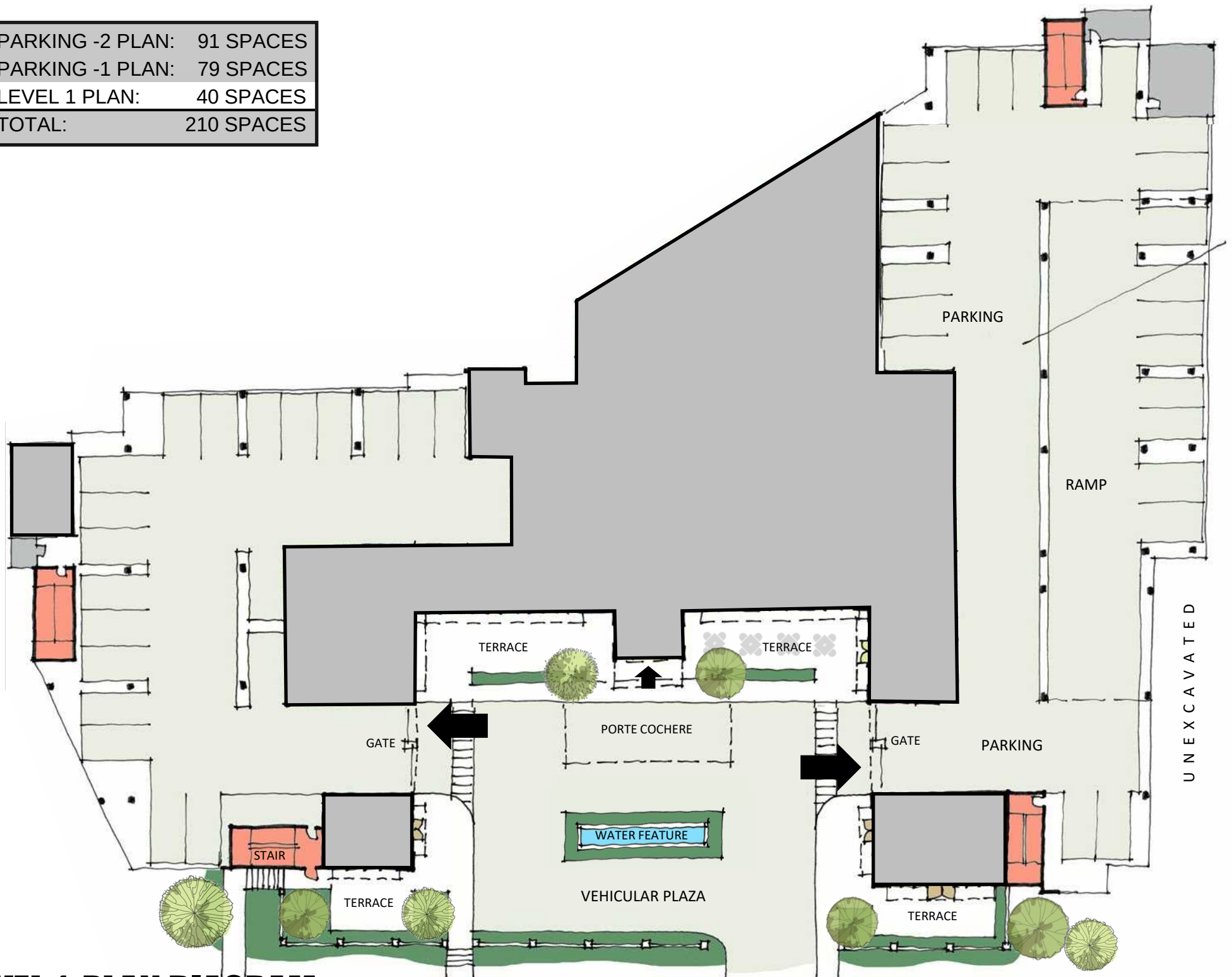
LEVEL 1 PLAN DIAGRAM
